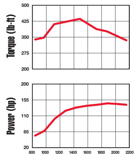
140 HP/434@1500 FR 91157
