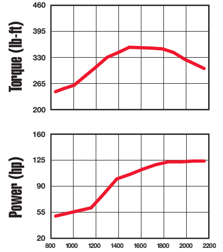
125 HP/355@1500 FR 91161
